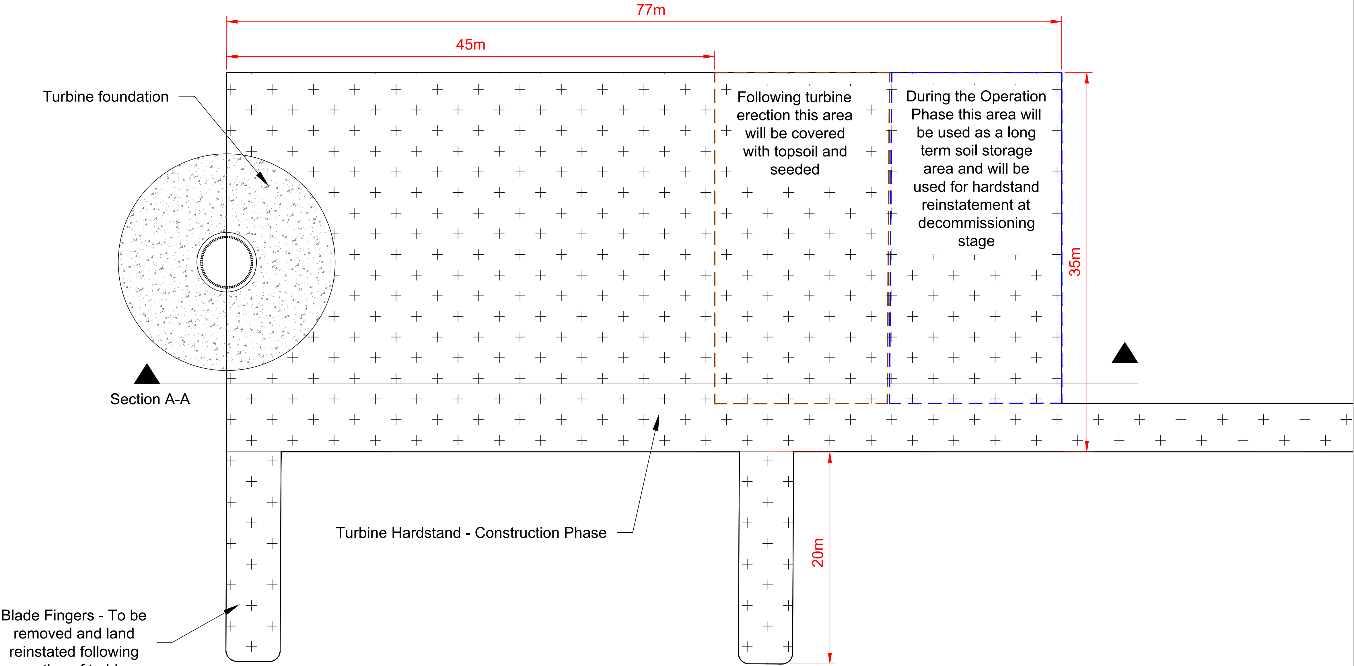
Turbine Hardstand - Plan view
